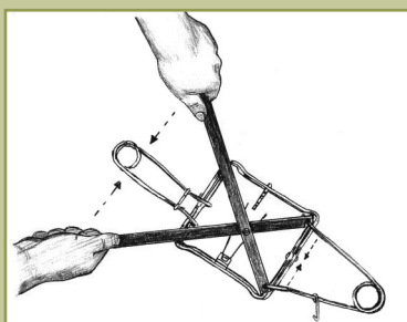
Figure NT3b. Using setting tool
